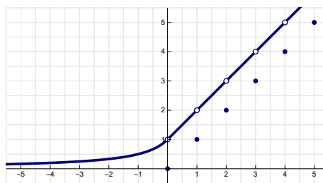
FIG. 24. A bijection \mathbb{R} \rightarrow \mathbb{R}_{\geq 0}
